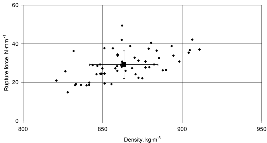
Fig. 2. – Relation between rupture force and density for briquettes stored in closed heated room in plastic net bag (sample C in Fig. 3; standard deviation is demonstrated by the line segments)
