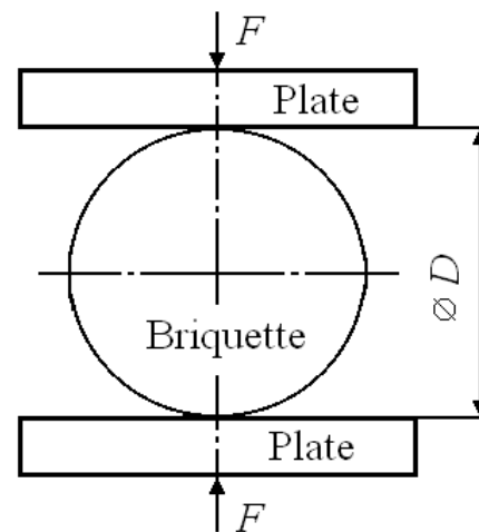
Fig. 1. – Principle of the plate-loading test
