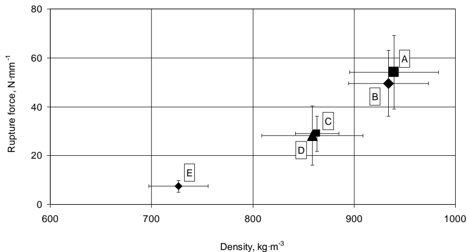
Fig. 3. – Relation between rupture force and density for all tested briquettes (standard deviation is demonstrated by the line segments): sample A – without exposure; sample B – storage space I, plastic bag; sample C – storage space I, plastic net bag; sample D – storage space II, plastic bag; sample E – storage space II, plastic net bag
